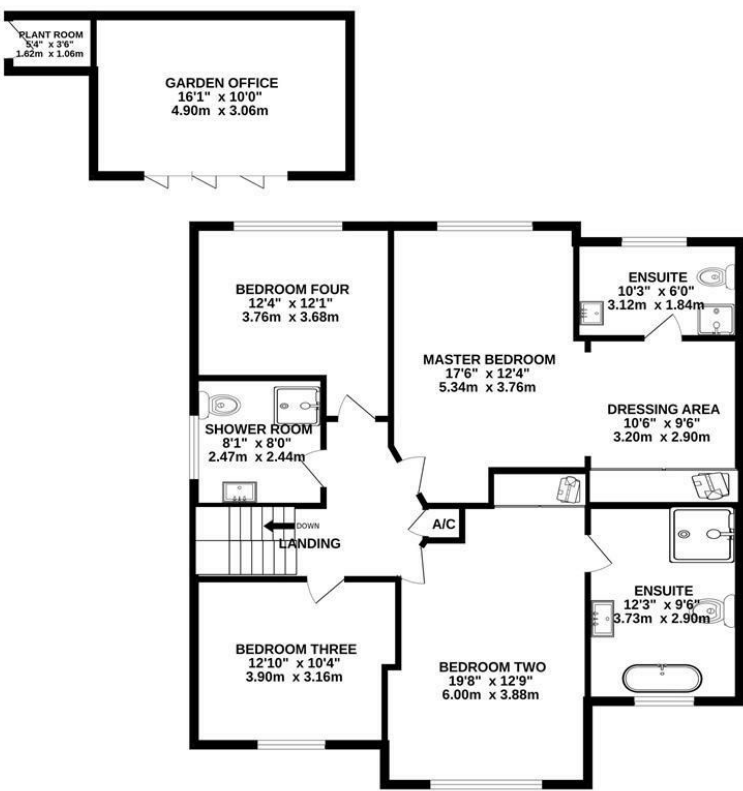
1ST FLOOR 1286 sq.ft. (119.5 sq.m.) approx.
